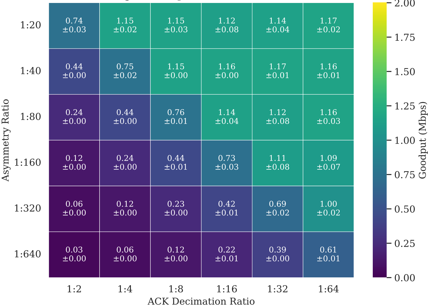
Averaged Goodput Overview (Loss 1%)
