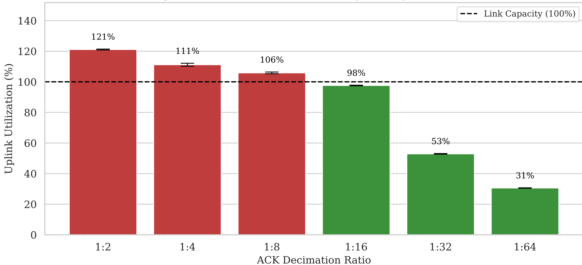
Averaged Reverse Path Saturation (Asymmetry 1:80, Loss 1%)
