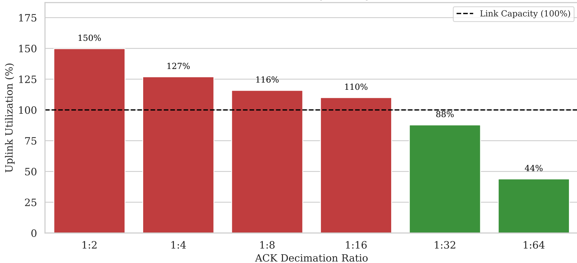
Reverse Path Saturation (Asymmetry 1:320, Loss 0%)
