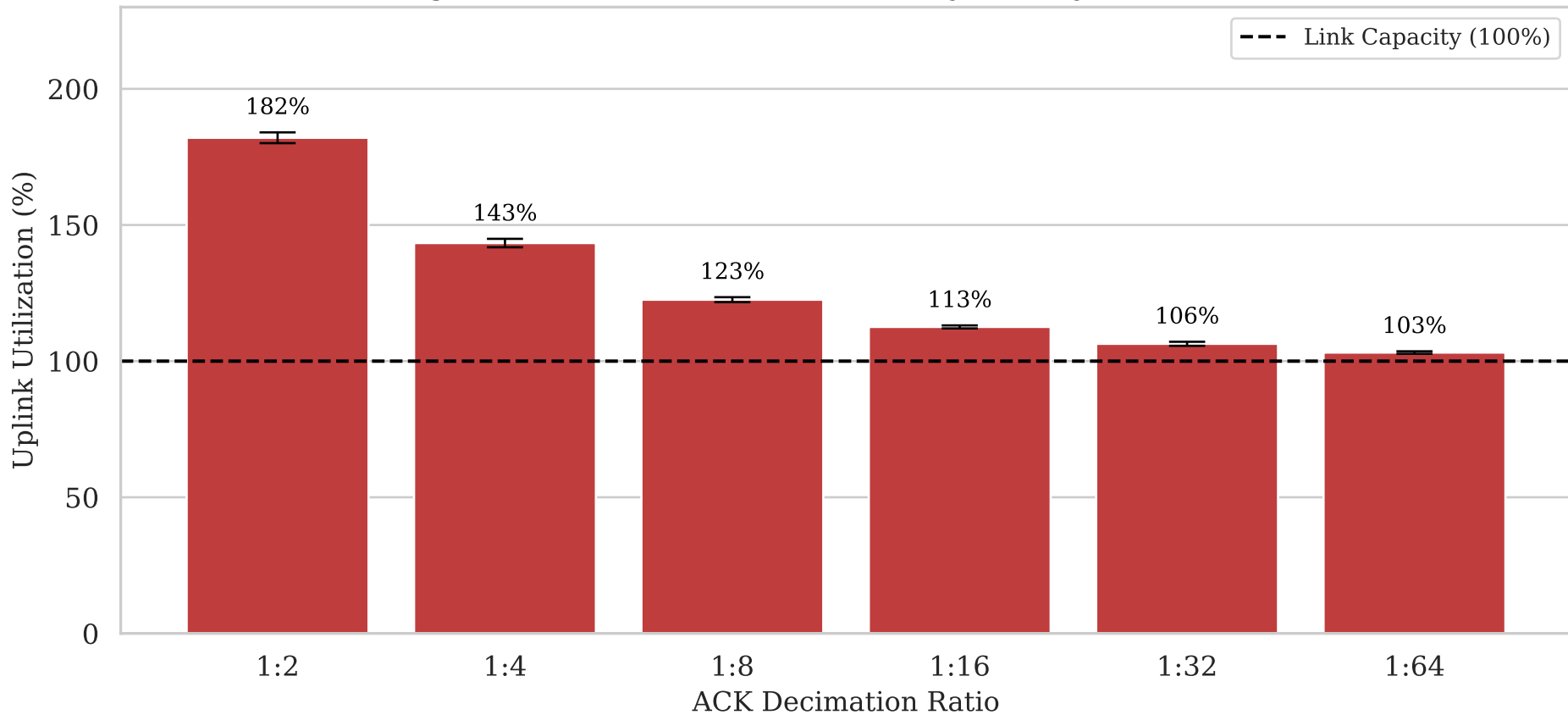
Averaged Reverse Path Saturation (Asymmetry 1:320, Loss 1%)
