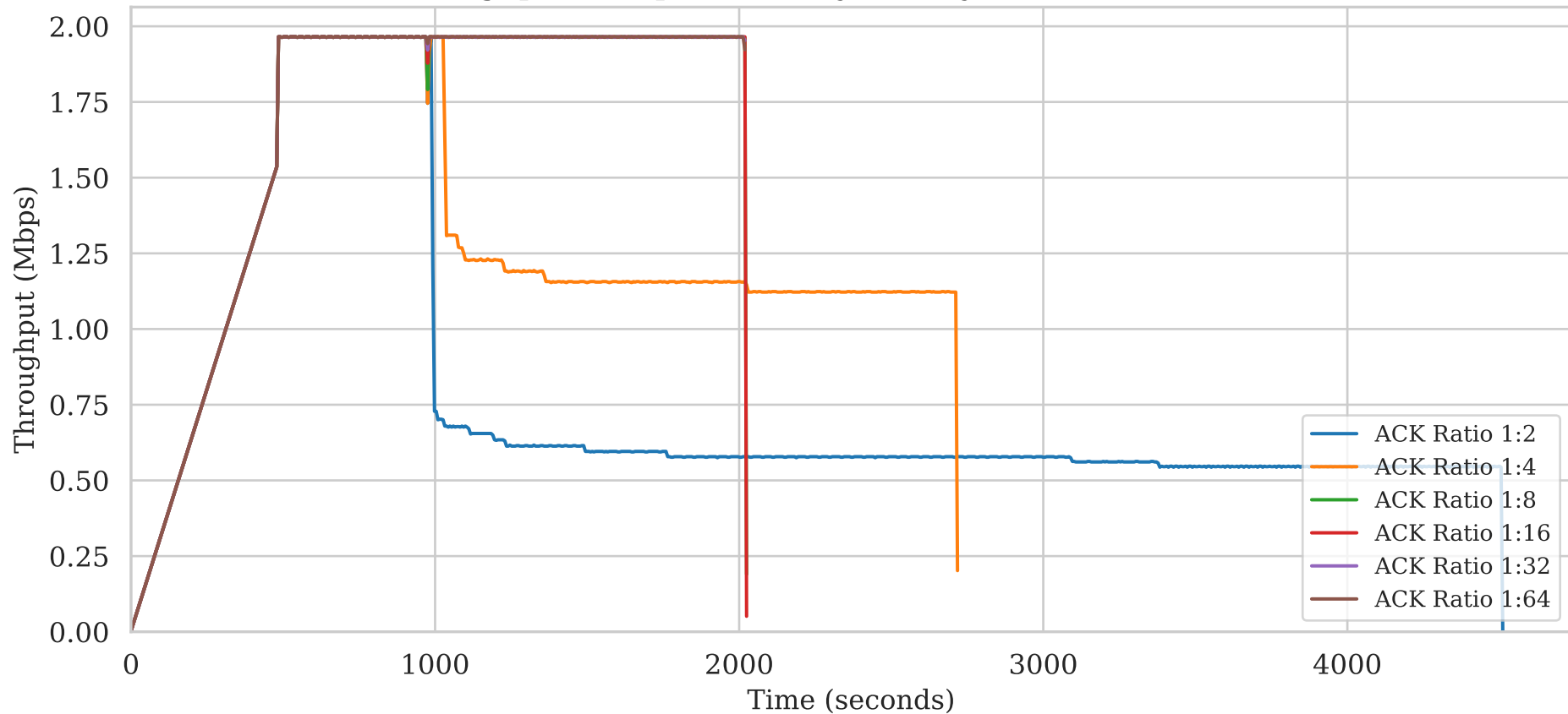
Throughput Comparison (Asymmetry Ratio 1:80, Loss 0%)
