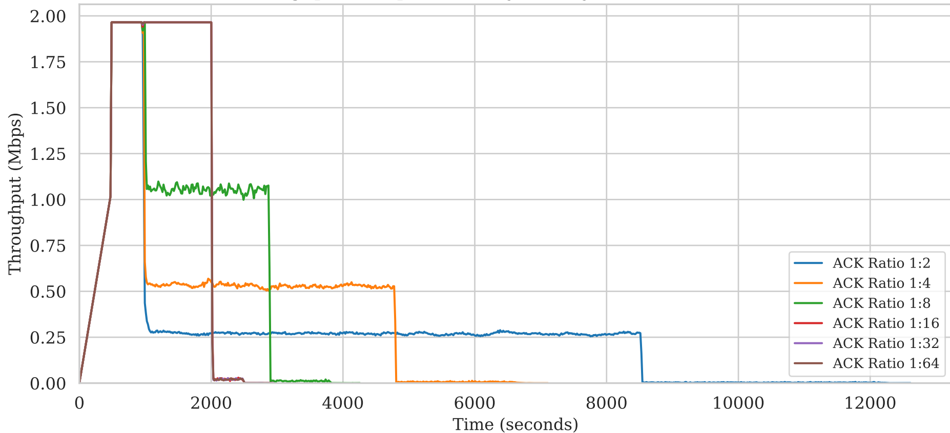
Throughput Comparison (Asymmetry Ratio 1:80, Loss 1%)
