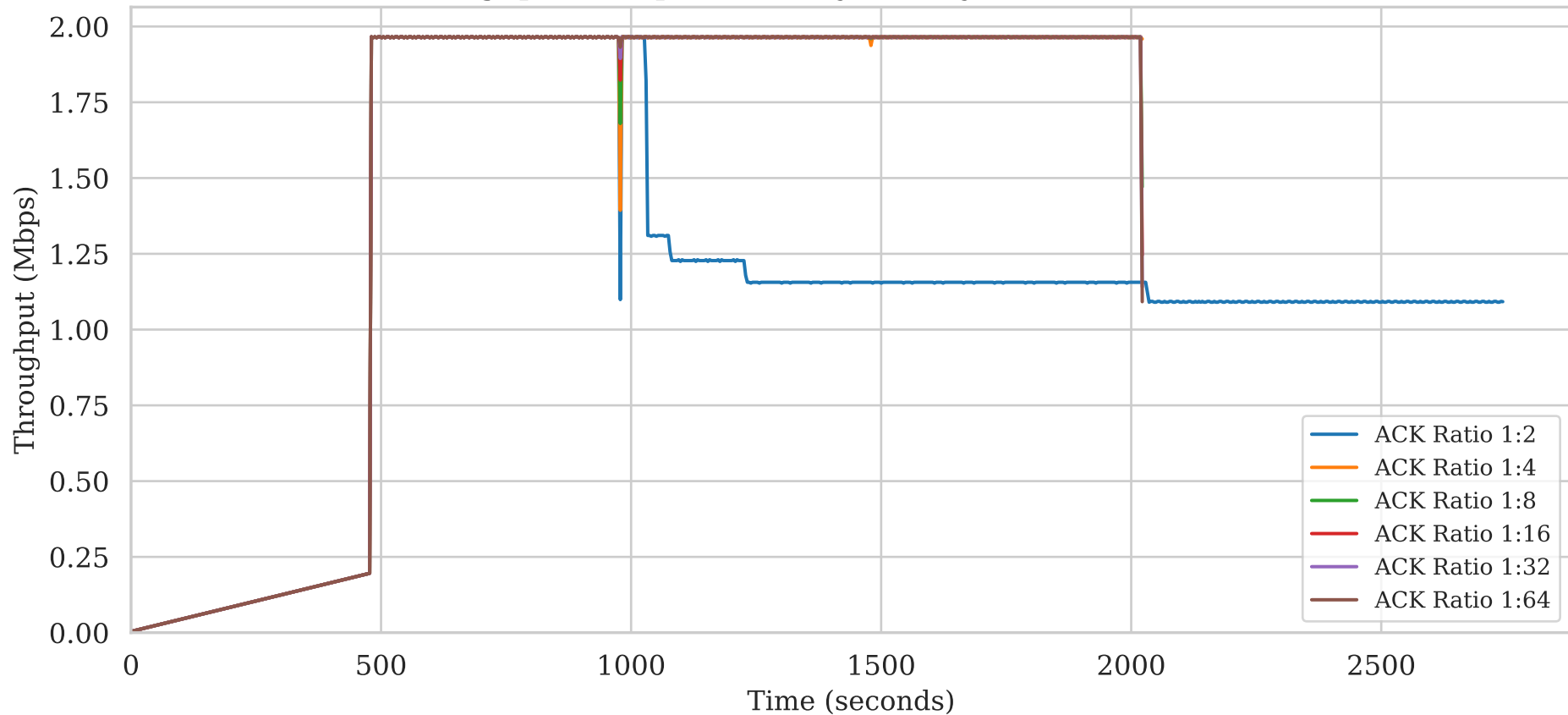
Throughput Comparison (Asymmetry Ratio 1:40, Loss 0%)
