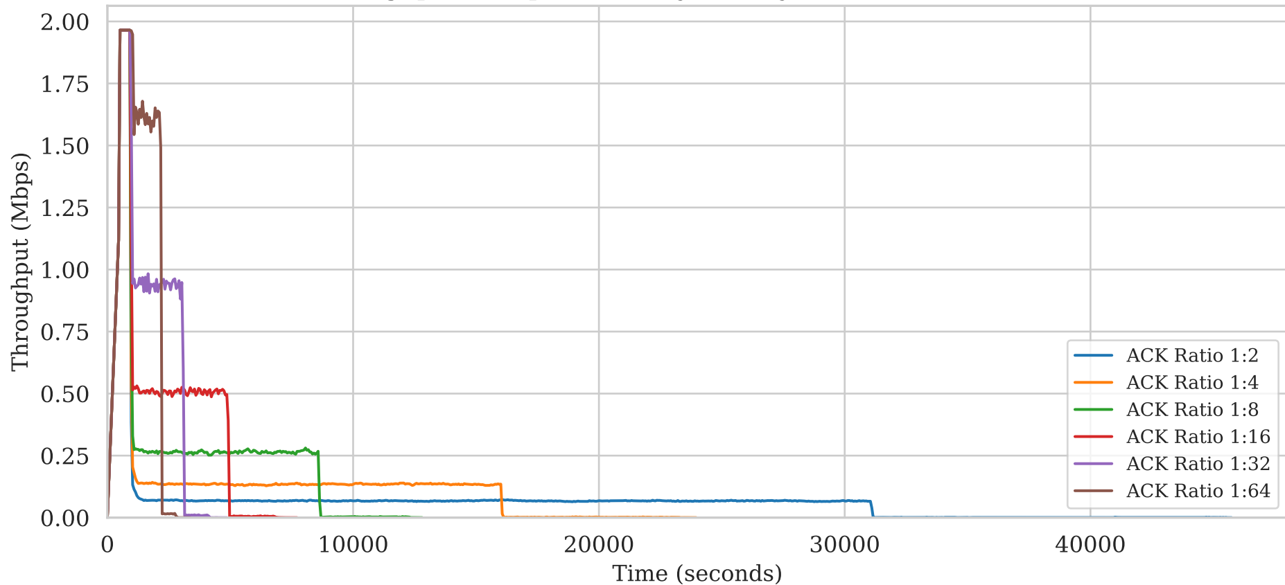
Throughput Comparison (Asymmetry Ratio 1:320, Loss 1%)
