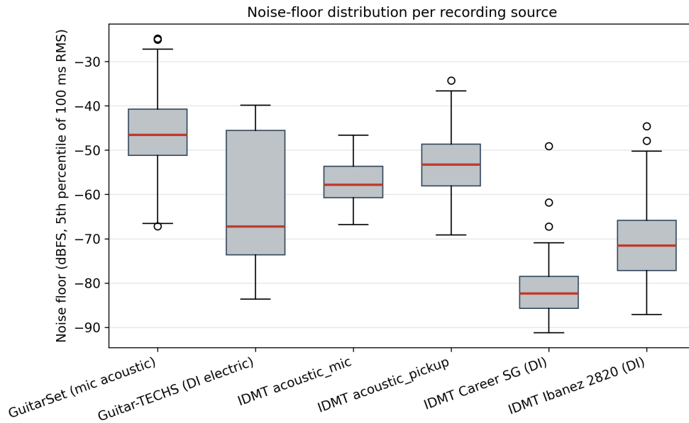
Figure 5.4: Per-source noise-floor distribution across the source recordings of the consolidated guitar corpus (box-plots; n = 360, 52, 128, 128, 123, 128 files respectively). Median noise floors range from −82.4 dBFS (IDMT Career SG DI) to −46.5 dBFS (GuitarSet mic-captured acoustic), a 35.9 dB spread that exceeds typical within-performance dynamic variation.
