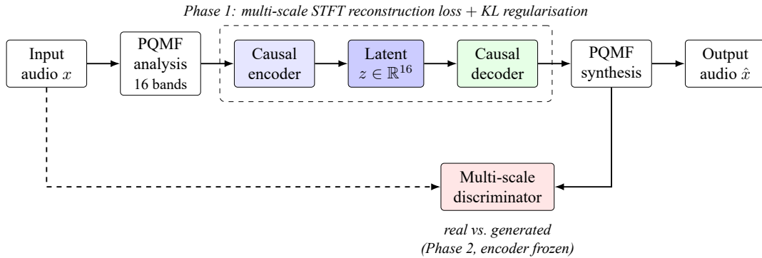
Figure 2.1: Simplified RAVE/BRAVE architecture and two-phase training. Input audio is split into 16 frequency bands by a PQMF analysis bank, encoded by a causal convolutional encoder into a low-dimensional Gaussian latent z , and reconstructed by a causal decoder followed by PQMF synthesis. In Phase 1 the encoder–decoder pair is trained to minimise a multi-scale STFT reconstruction loss with KL regularisation of the latent; in Phase 2 the encoder is frozen and the decoder is fine-tuned adversarially against a multi-scale discriminator. BRAVE differs from standard RAVE chiefly in using causal convolutions and a reduced compression ratio to enable sub-10 ms streaming inference.
