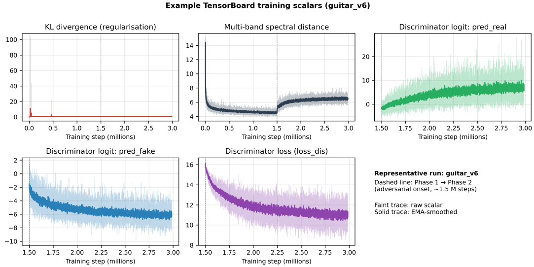
Figure C.1: Example TensorBoard training scalars for the canonical guitar_v6 run: KL regularisation, multi-band spectral distance, the two discriminator logits ( pred_real , pred_fake ) and the total discriminator loss. The dashed vertical line marks the Phase 1→Phase 2 transition (~1.5 M steps); faint traces are the raw scalars and solid traces an exponential moving average. This is the dashboard view from which the diagnostic signatures of Chapter 5 are read.
