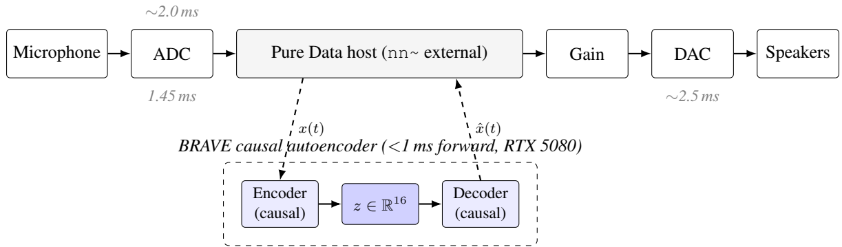
Figure 3.1: Block diagram of the real-time voice-to-instrument resynthesis pipeline. The Pure Data host invokes the BRAVE causal autoencoder via the nn~ external ; the encoder maps each block of audio x(t) to a 16-dimensional latent z and the decoder regenerates \hat{x}(t) in the target-instrument timbre. Latency contributions per stage are listed in Table 3.1.
