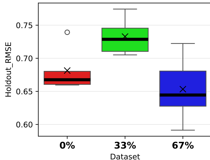
Holdout RMSE
