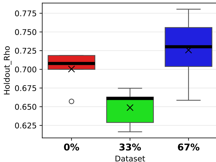
Holdout \rho
