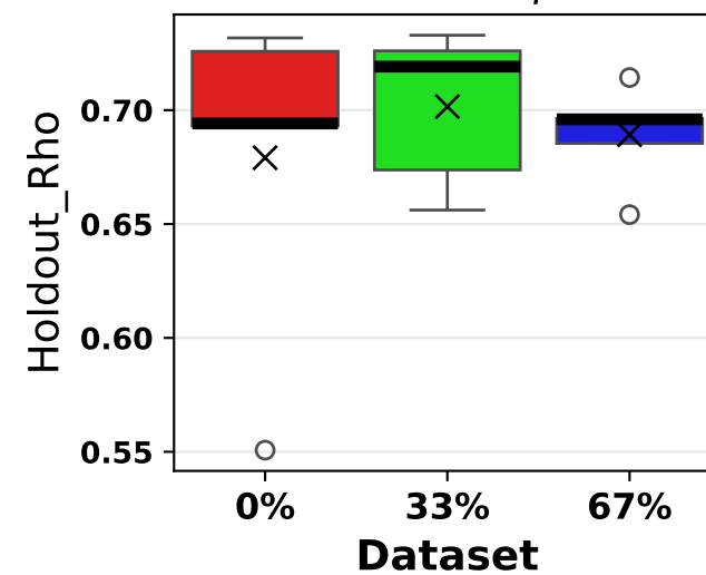
Holdout \rho
