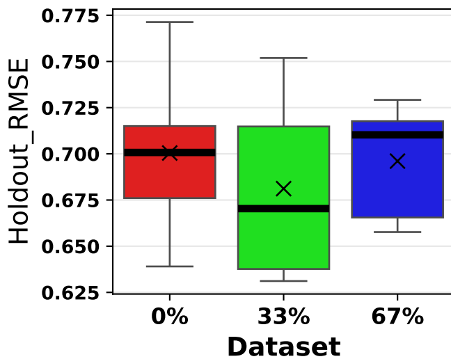
Holdout RMSE
