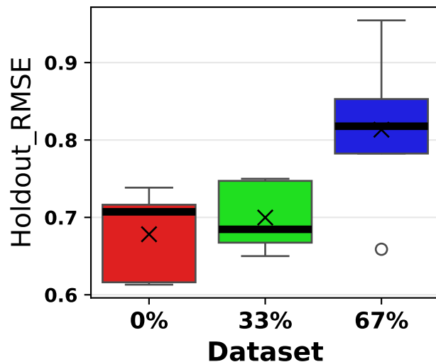
Holdout RMSE
