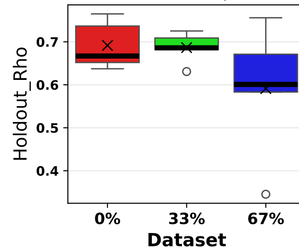
Holdout \rho
