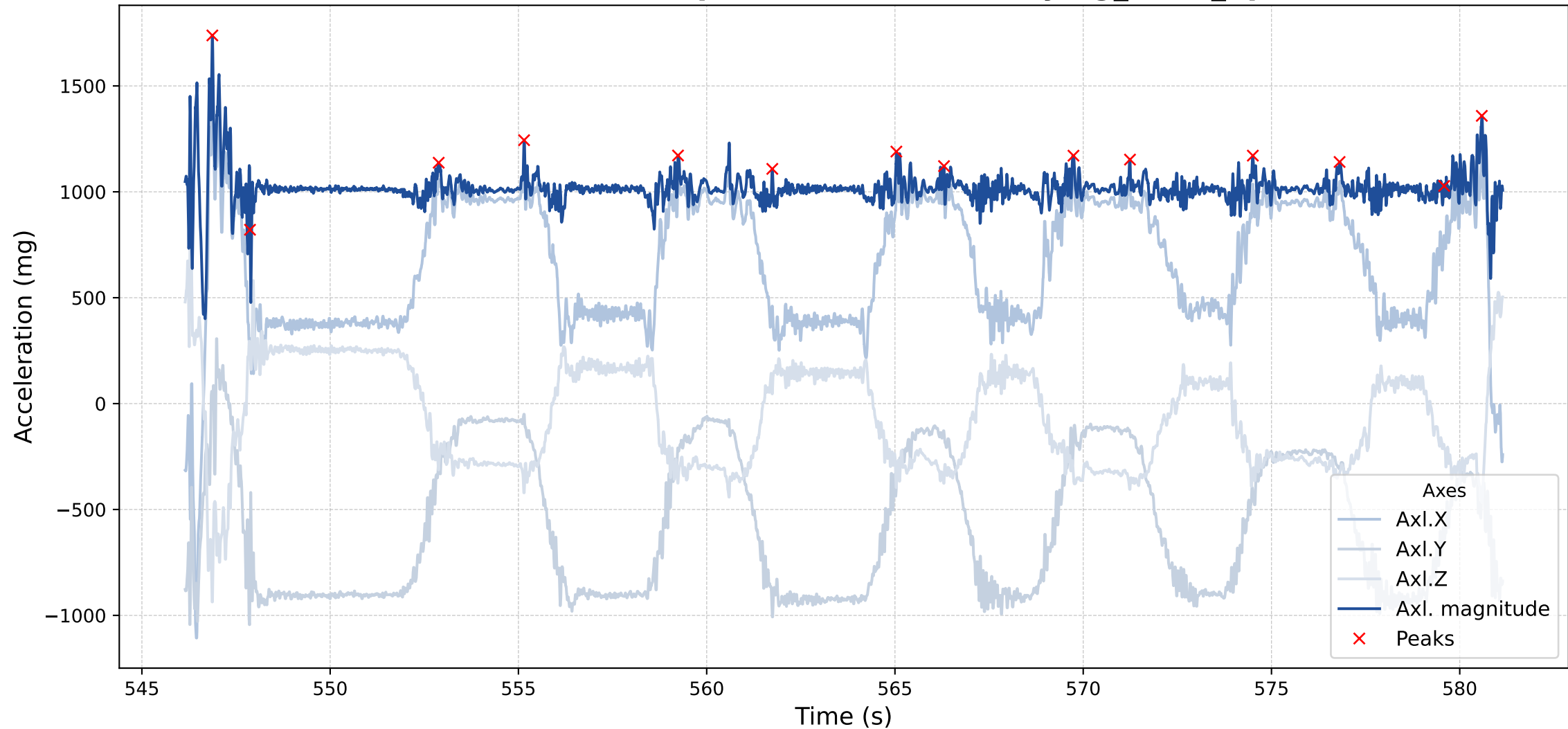
Acceleration Components over Time (lying_arms_up)
