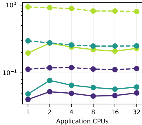
CMG setup
