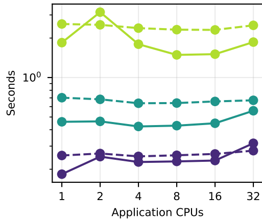
Setup + solve
