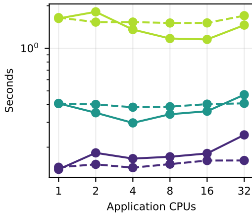
PCG solve
