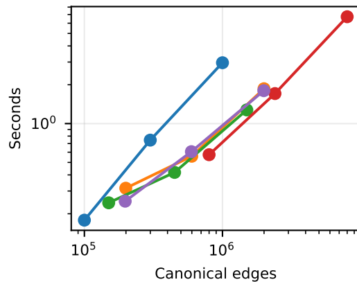
Rust: Setup + solve
