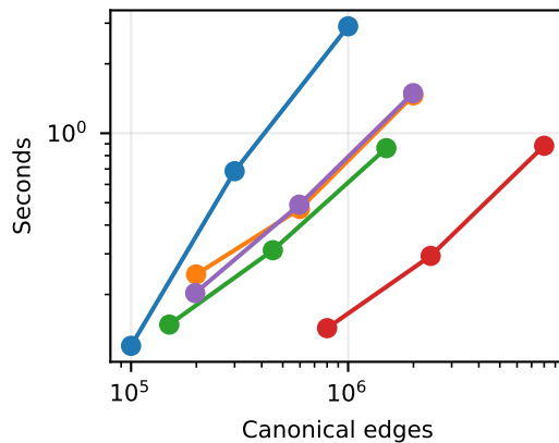
Rust: PCG solve
