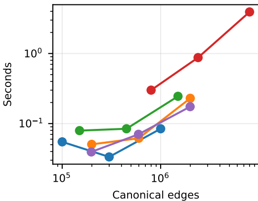
Rust: CMG setup
