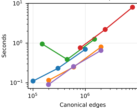
Matlab: CMG setup
