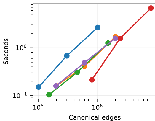
Matlab: PCG solve
