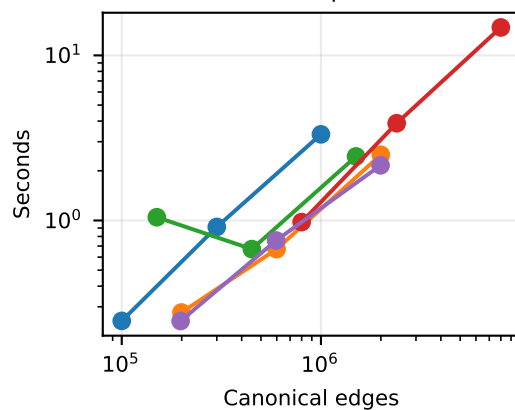
Matlab: Setup + solve
