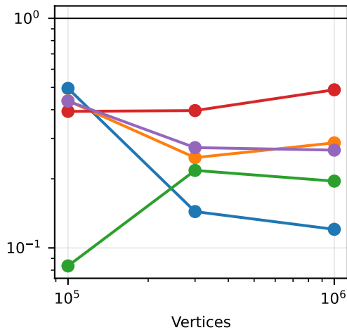
CMG setup
