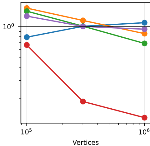
PCG solve
