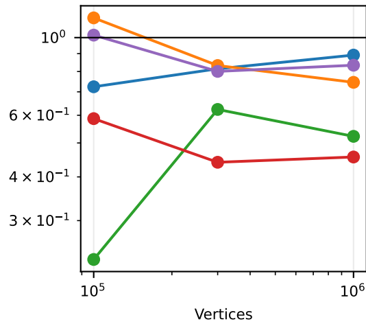
Setup + solve
