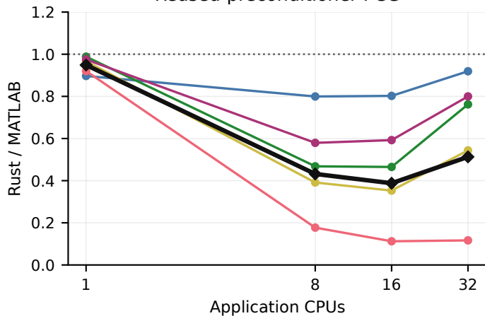
Reused-preconditioner PCG
