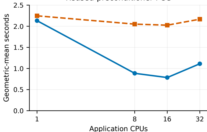
Reused-preconditioner PCG
