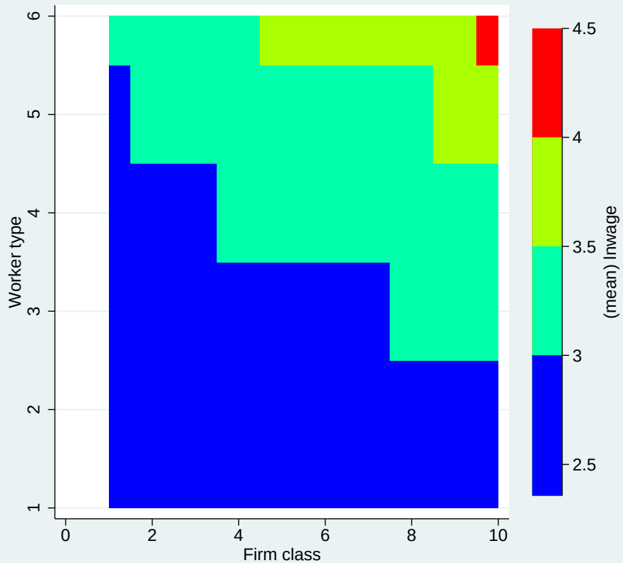
Realized mean log earnings
