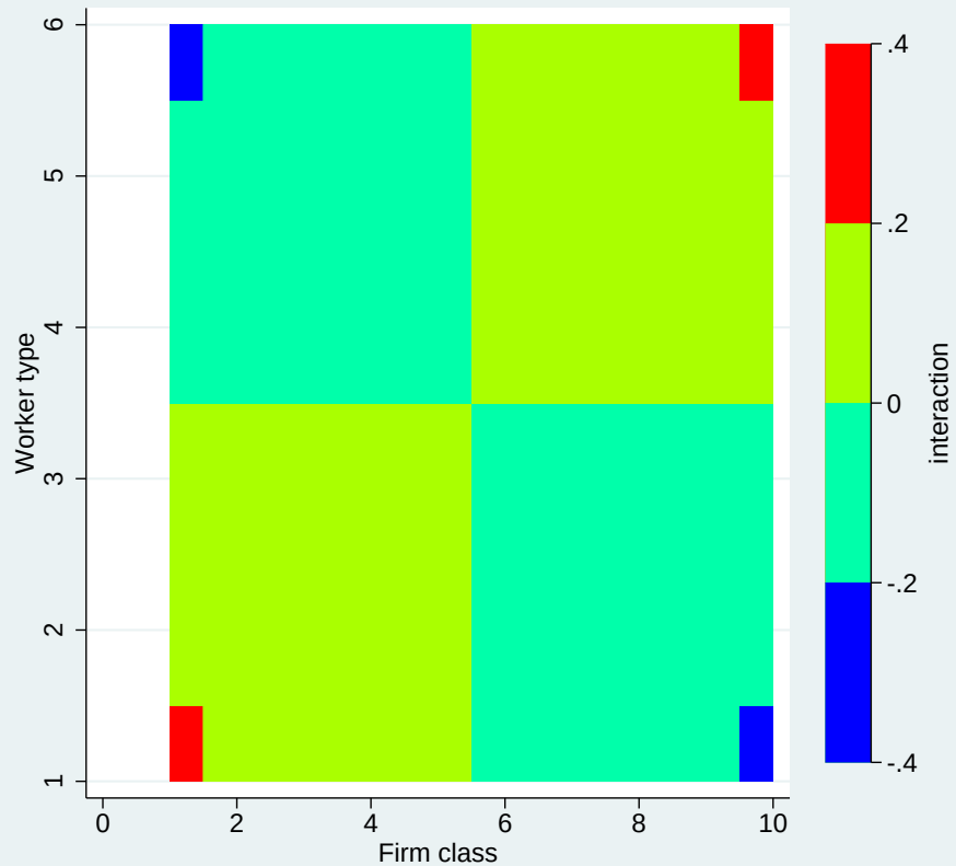
Nonadditive cell location
