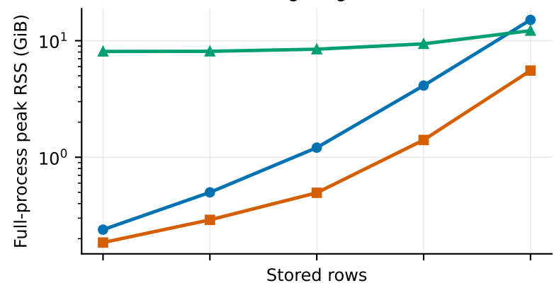
Strong, degree 6
