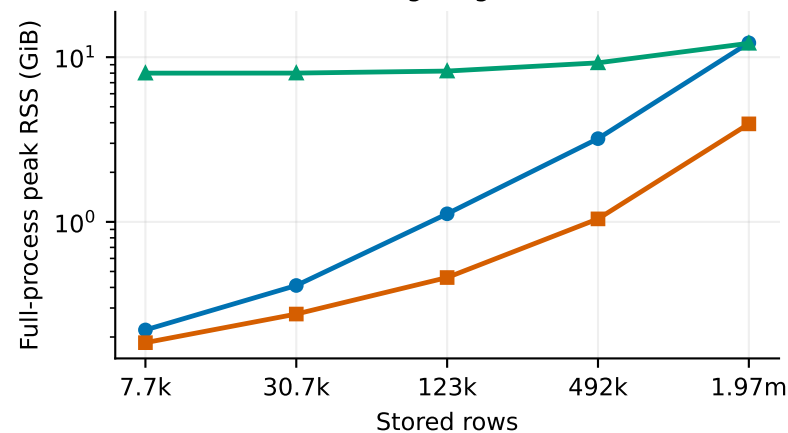
Strong, degree 6
