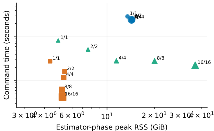
Shallow-tree bottleneck, degree 3
