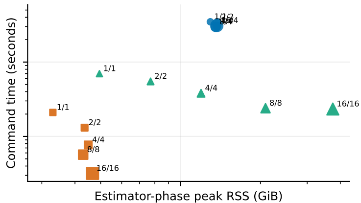
Shallow-tree bottleneck, degree 3
