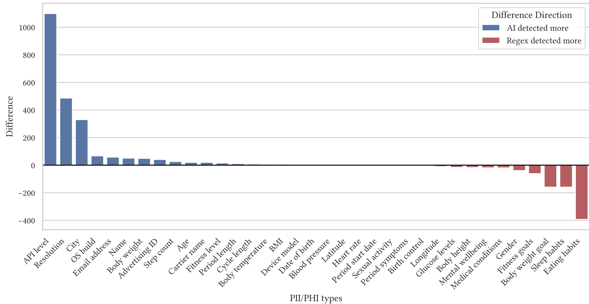
AI Performance vs. Regex (Positive = AI detected more)
