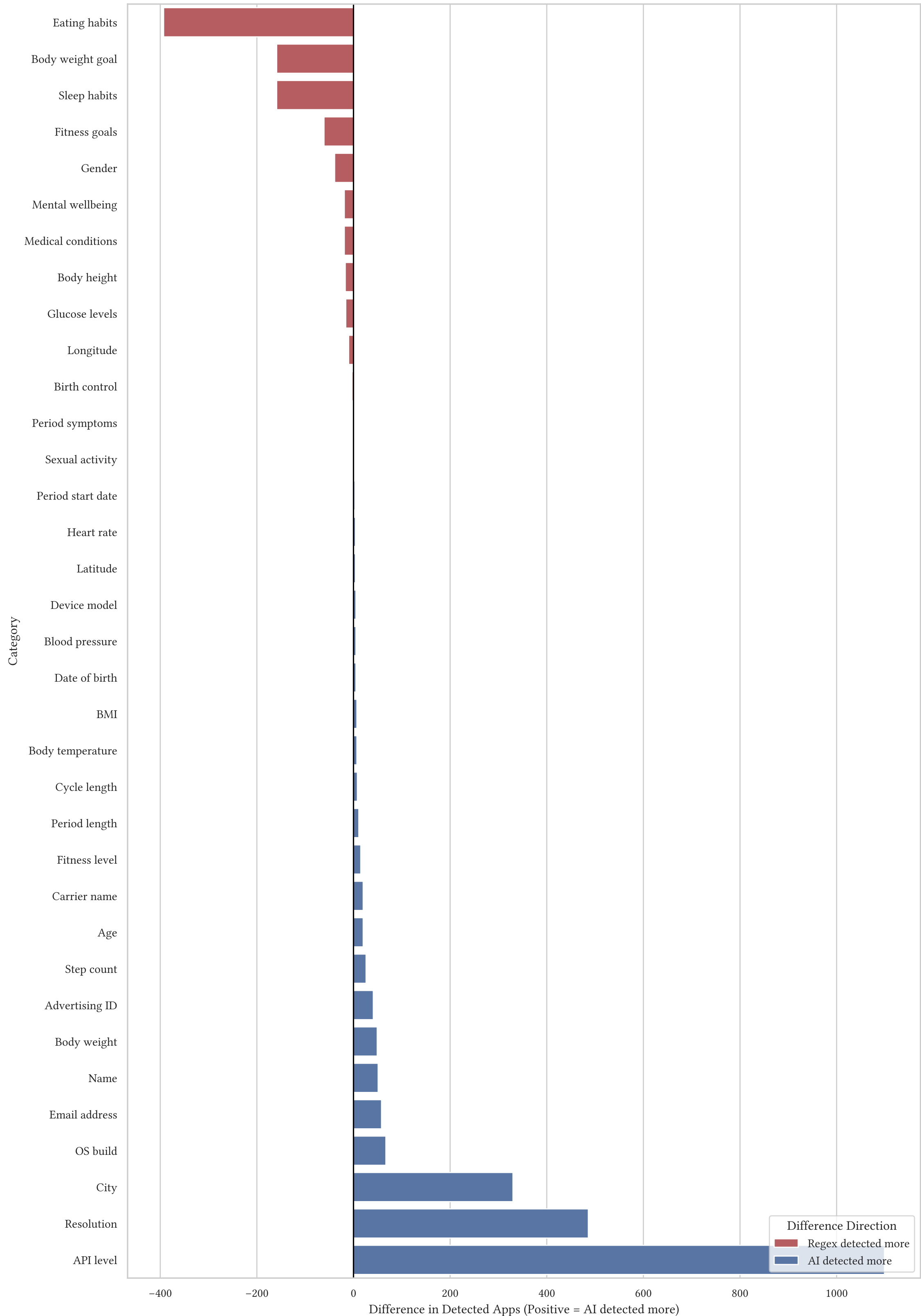
Diverging Bar Chart: AI Performance vs. Regex ( \Delta = \text{AI} - \text{Regex} )
