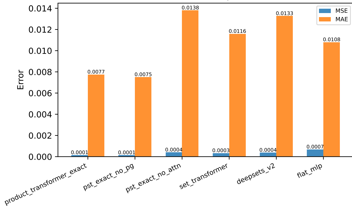
MSE / MAE Comparison
