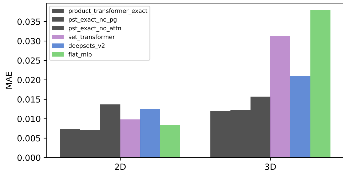
MAE by Dimension
