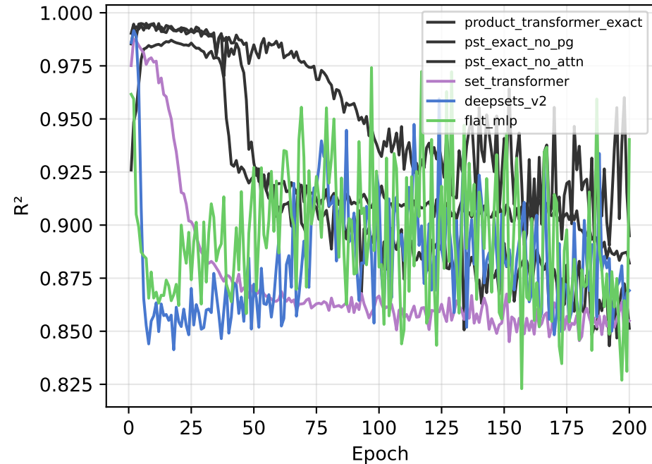
Val R 2
