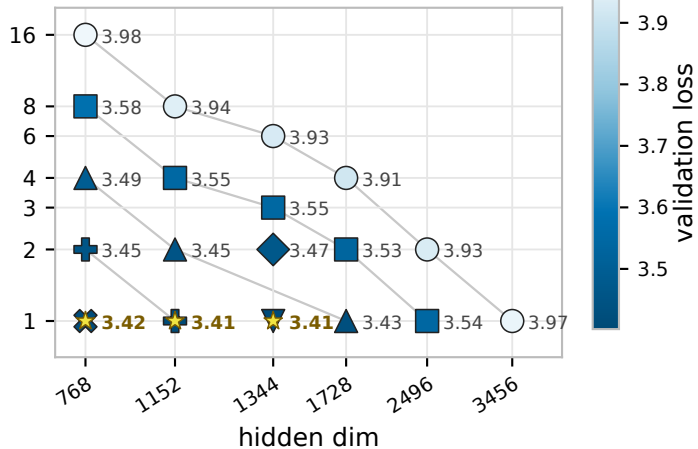
PRE Transformer, segment 2048
