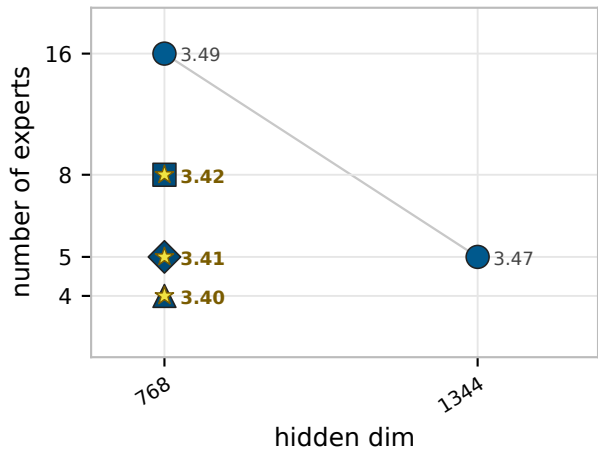
PRE Recurrent Transformer, memory 2048
