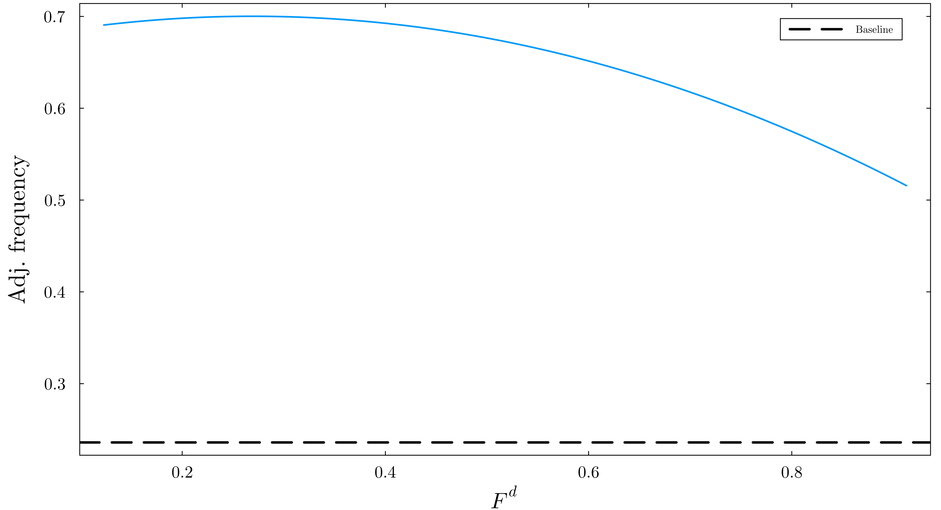
Effect of F^d on Adj. frequency
