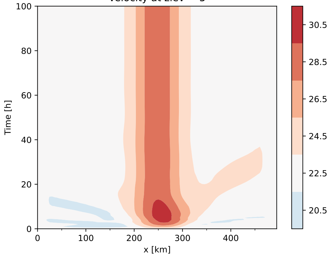
Velocity at zlev = 5
