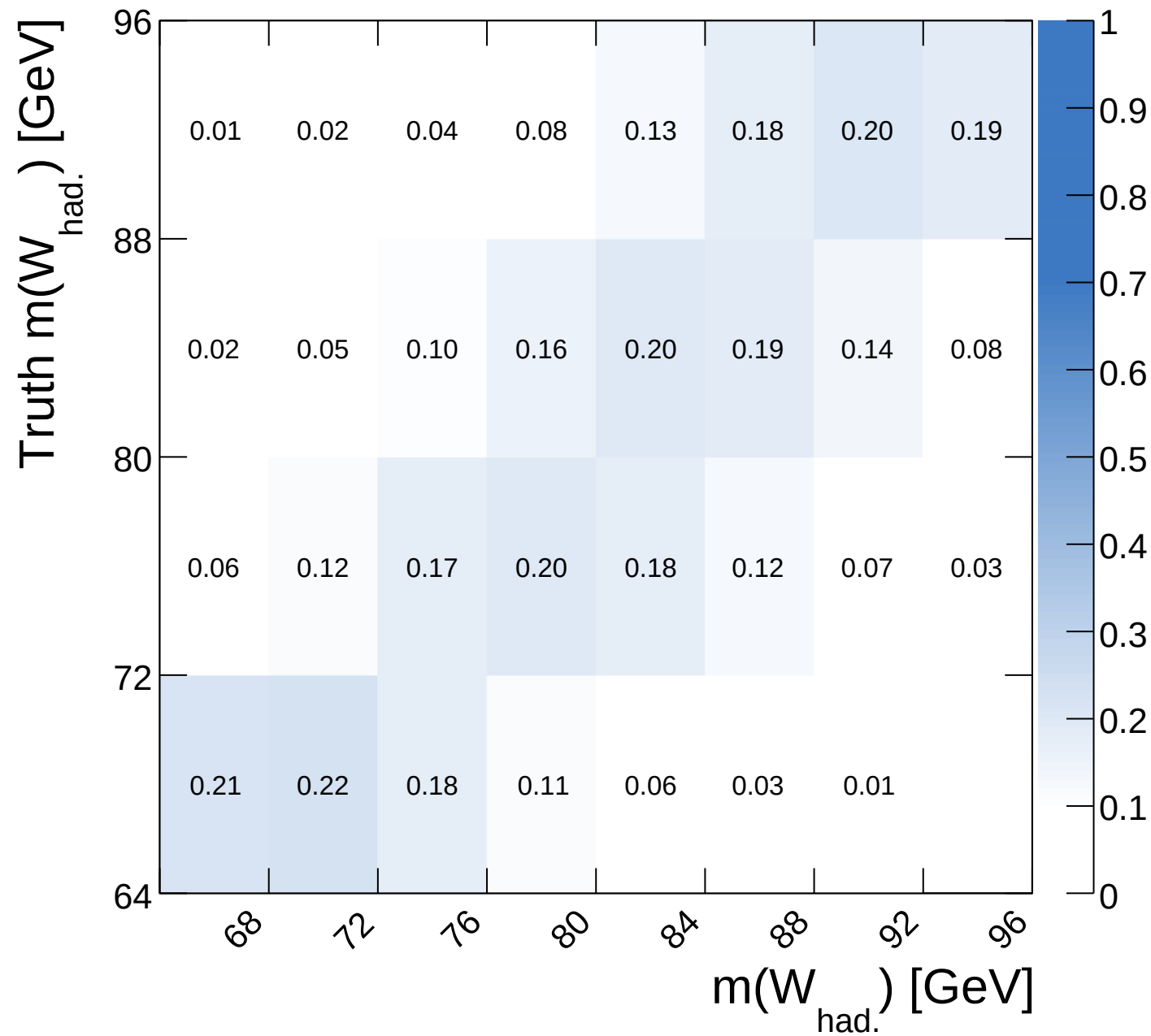
Nominal \sqrt{s} = 13 \text{ TeV}, 140 \text{ fb}^{-1} migration matrix
