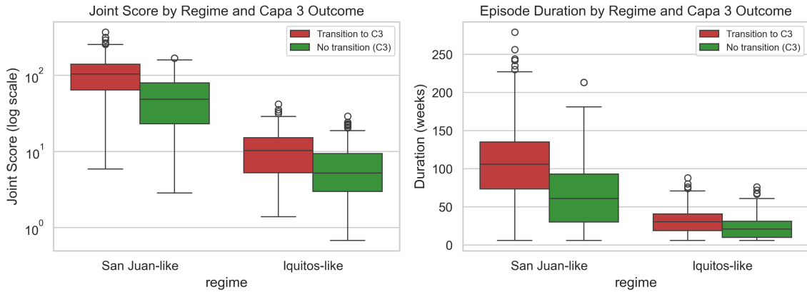
Figure 2: Ontological contrast between dynamical regimes (synthetic data). Boxplots of Joint Score (log scale, left) and episode duration (right) for synthetic Joint episodes, stratified by regime (San Juan-like vs. Iquitos-like) and by transition to Layer 3. San Juan-like episodes are substantially longer and higher-intensity, with clear separation by outcome. Iquitos-like episodes are short and weak, showing minimal differentiation—consistent with intrinsically rare sustained Layer 2 states.
