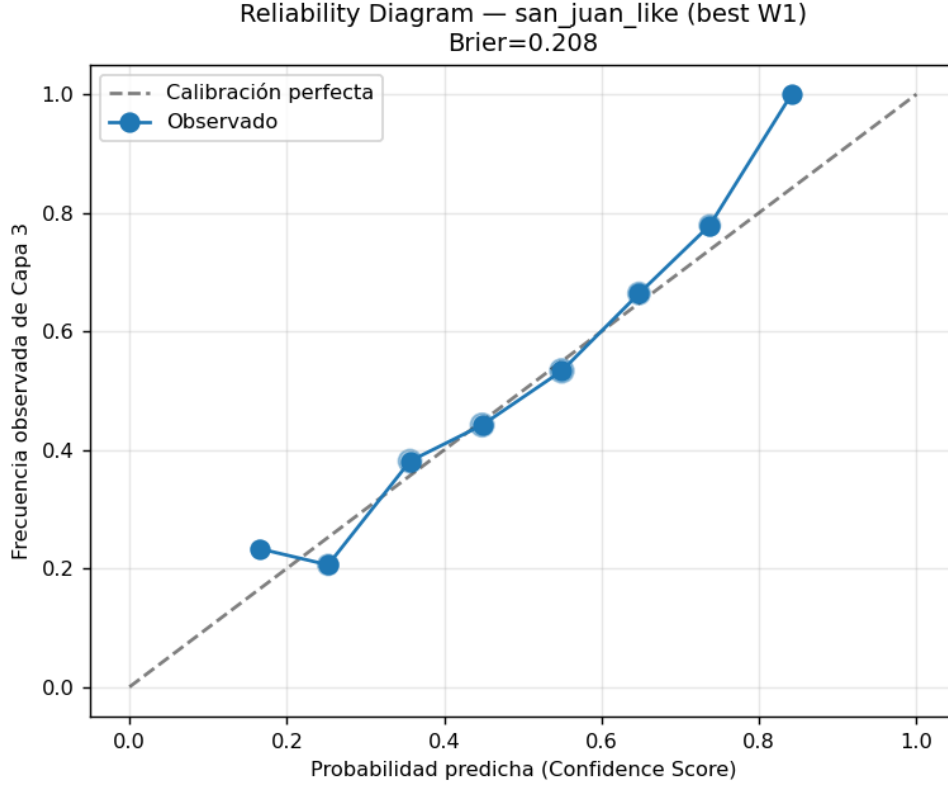
Figure 3: Calibration (reliability) diagram for the San Juan-like regime under the recommended weight vector. Observed frequency of Layer 3 transition is plotted against binned predicted Confidence Score. Points close to the diagonal indicate good calibration, with modest recoverable bias.
