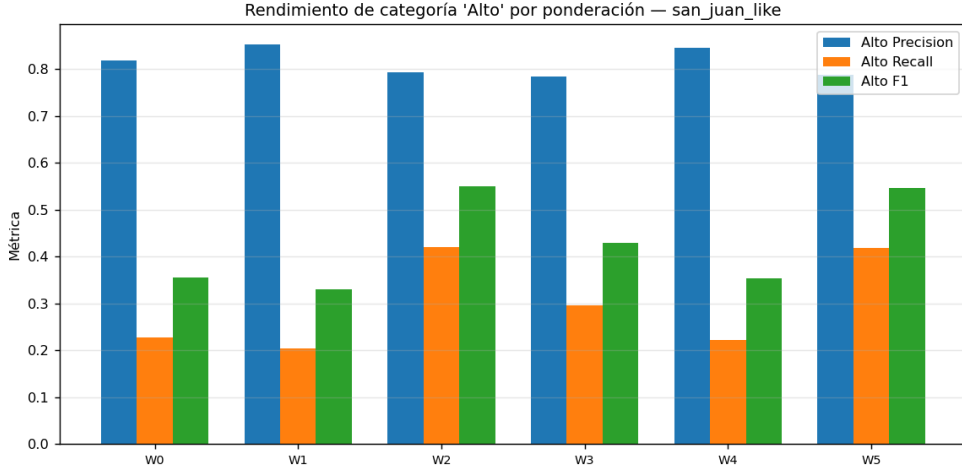
Figure 4: Performance of the “Alto” category under the recommended weight vector in the San Juan-like regime. The categorization concentrates episodes with elevated empirical transition rates. The Iquitos-like regime produced virtually no “Alto” episodes, confirming that high-confidence Joint episodes are regime-dependent.
