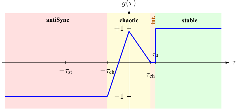
Figure 3: Schematic of operational bands on the \tau -axis and the piecewise gate g(\tau) from Equation (7). Note the asymmetric treatment of the anti-synchronous ray ( g = -1 ) relative to the positive intermediate band ( g = 0 ).
