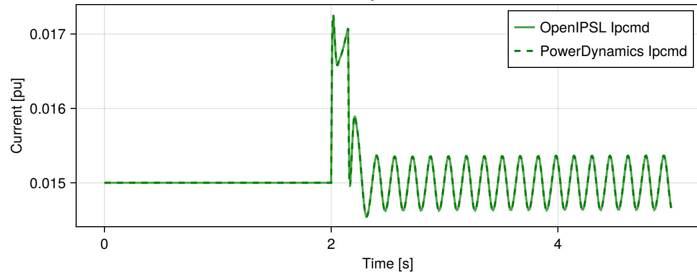
PlantController: Qext &amp; Pref
