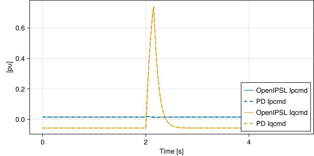
regca: I_p & I_q (final outputs)
