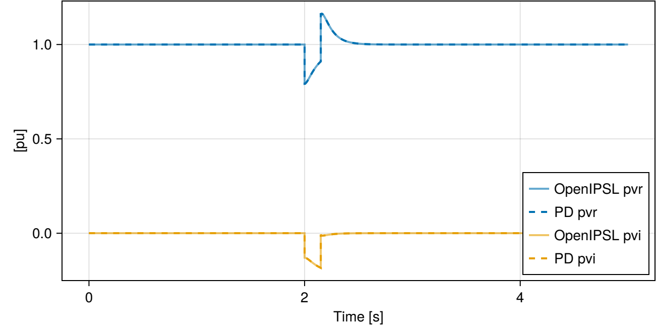
Terminal: pvr & pvi
