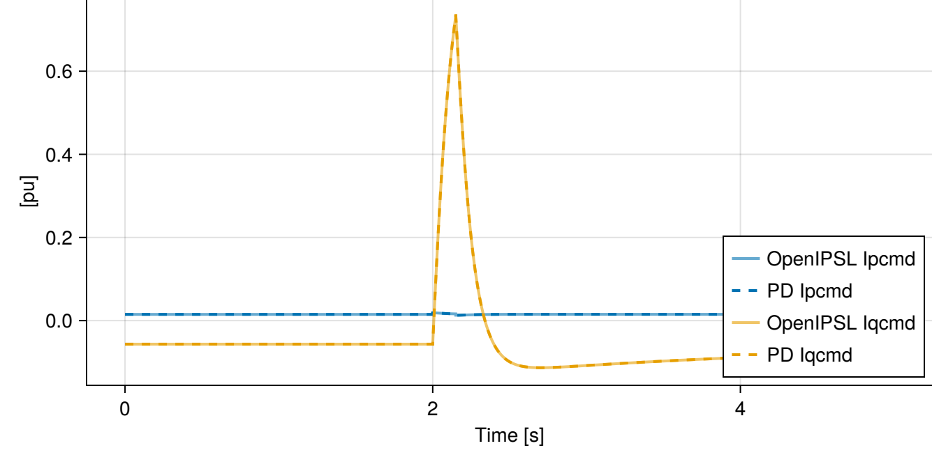
regca: I_p & I_q (final outputs)
