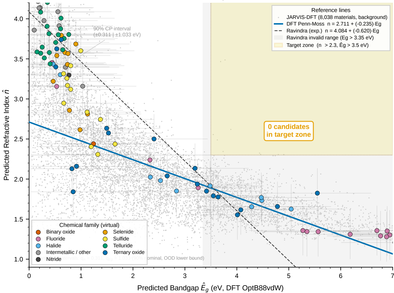
Fig. 2 | Virtual Screening: 106 Hypothetical Structures in (\hat{E}_g, \hat{n}) Space
