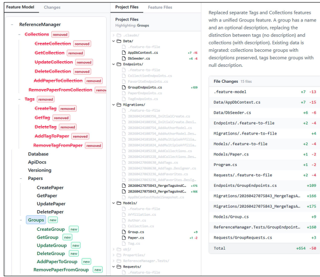
Figure 3: Agent-HANs dashboard. Left: feature tree with change indicators. Center: Project Files of the selected feature. Right: summary with line additions and deletions.
