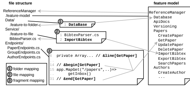
Figure 1: Embedded feature annotation system [31]
