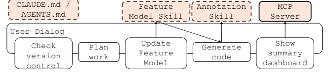
Figure 2: One Agent-HAnS cycle showing the stages the agent executes and involved components per step
