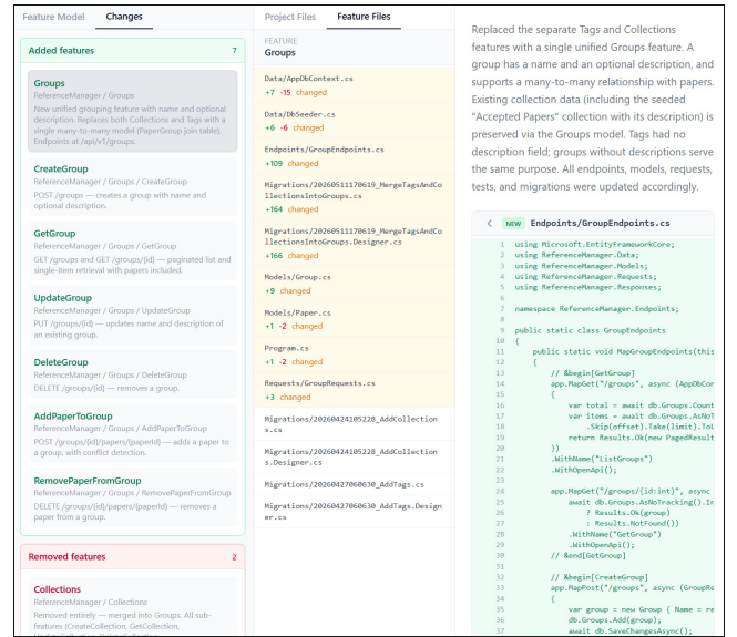
Figure 4: Agent-HANs dashboard (continued). Left: Changes tab with feature descriptions. Center: Feature Files for the selected feature. Right: file content for code inspection.
