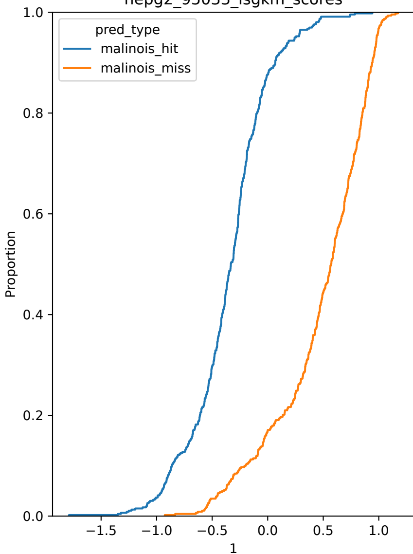
hepg2_95033_lsgkm_scores
