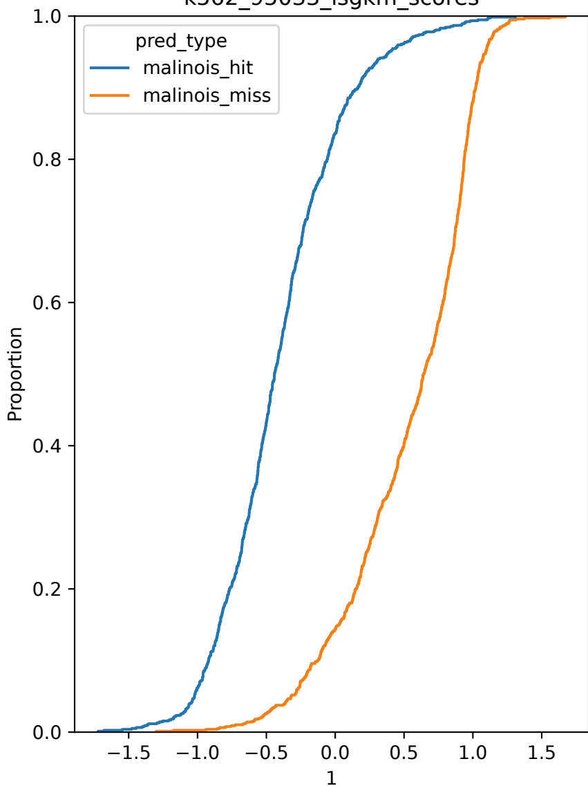
k562_95033_lsgkm_scores
