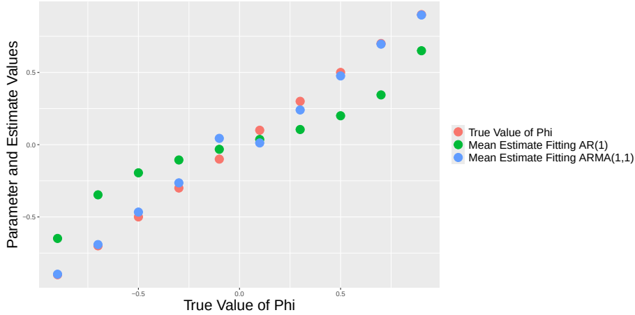
Figure 3: Aggregated estimates for AR. An interactive version of this figure is available here .
