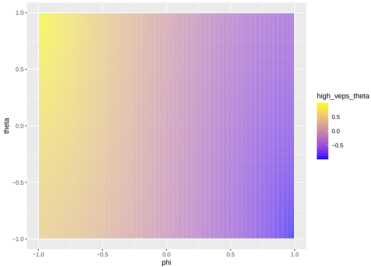
Theta Est. for Daily Variance 10x That of Time Series
