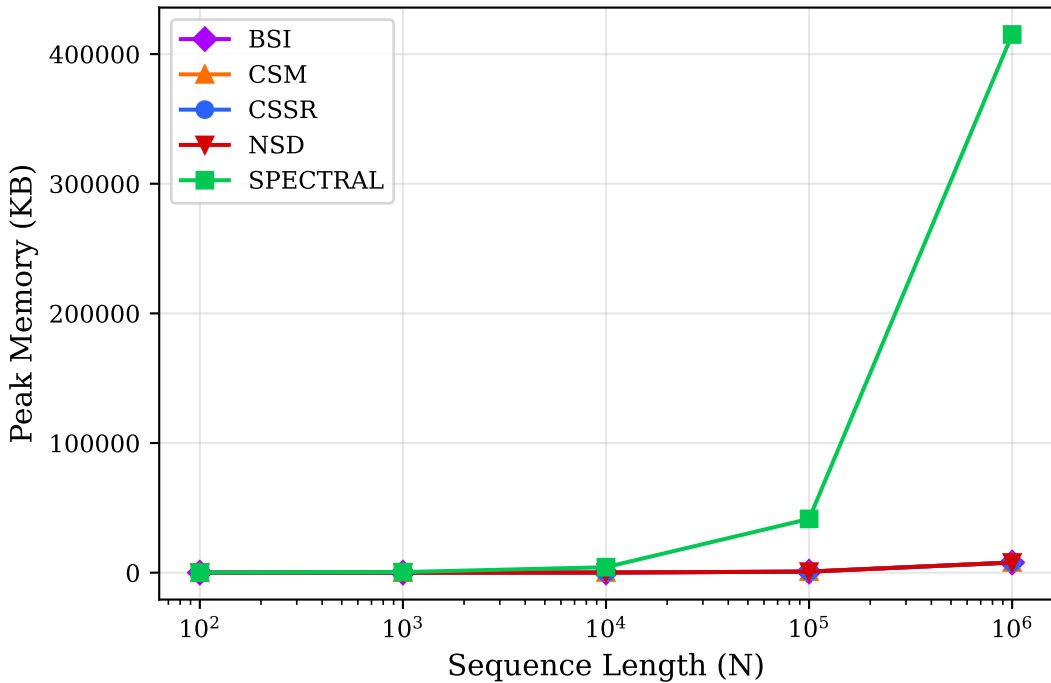
Memory Usage Scaling
