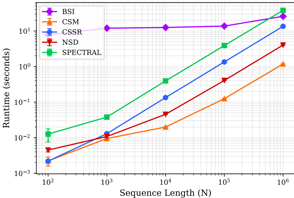
Inference Runtime Scaling (All Algorithms)
