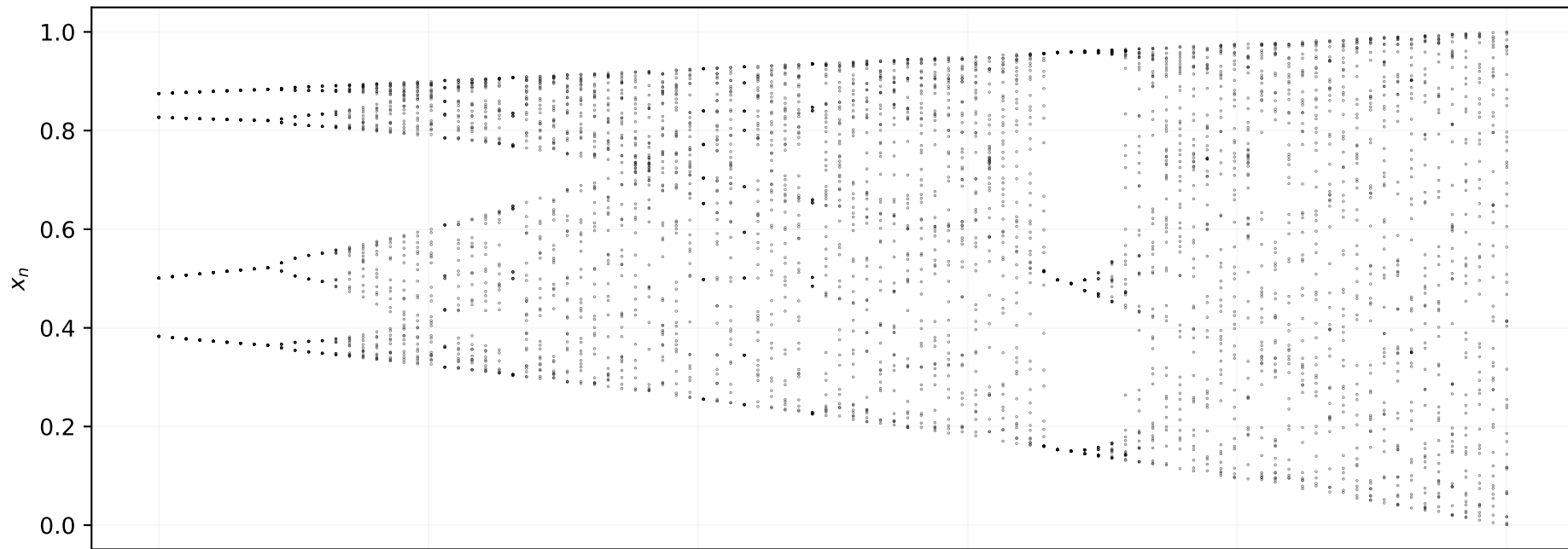
Logistic Map Bifurcation Diagram
