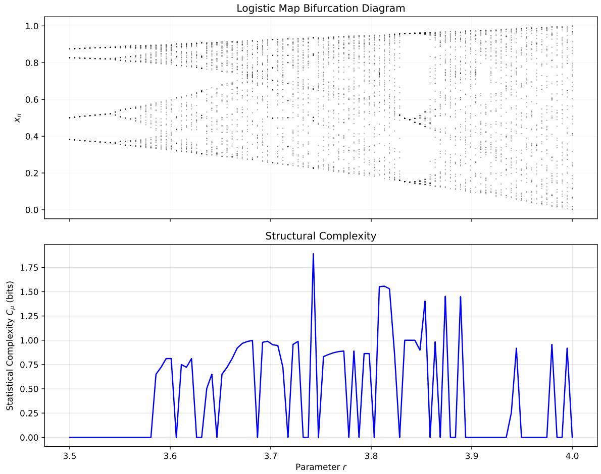
Figure 3: The Architecture of Chaos. Top: The bifurcation diagram (values of x ). Bottom: Structural complexity ( C_\mu ).
