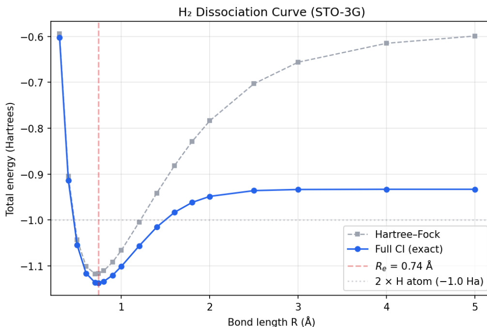
Figure 1: \text{H}_2 dissociation curve (STO-3G): Hartree–Fock vs Full CI. The FCI curve correctly dissociates while HF fails at large bond lengths.
