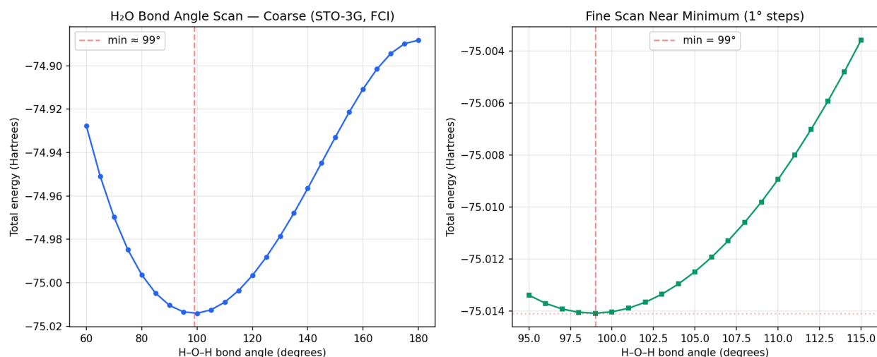
Figure 2: H 2 O bond angle scan (STO-3G, FCI): coarse scan (left) identifies the minimum near 100°; fine scan (right) pinpoints it at 99°.
