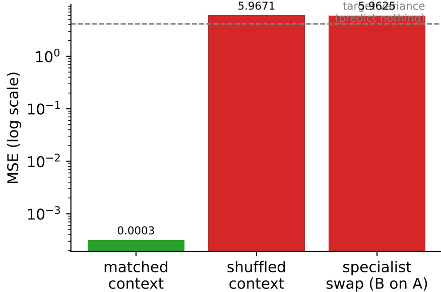
(a) Specialist is task-conditioned
