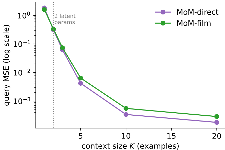
(b) Accuracy scales with information given
