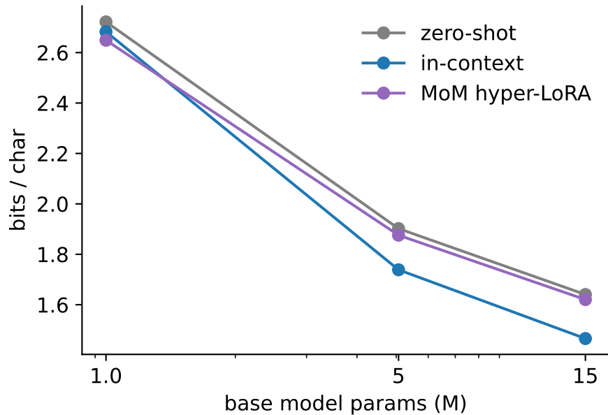
(a) enwik8 conditioning vs scale
