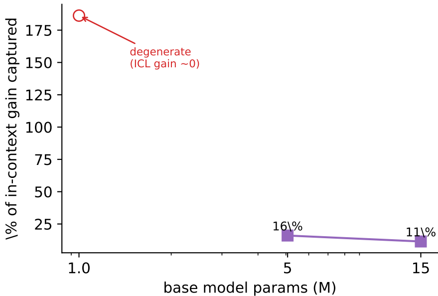
(b) Gap to in-context widens with scale
