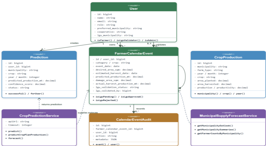
Harviana Class Diagram
