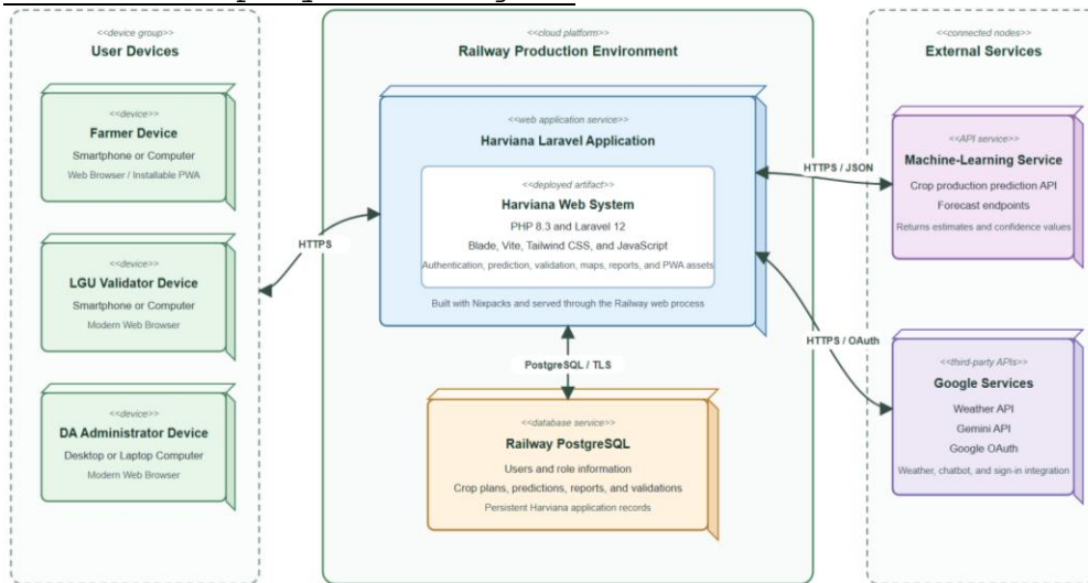
Figure 25 Harviana Deployment Diagram
