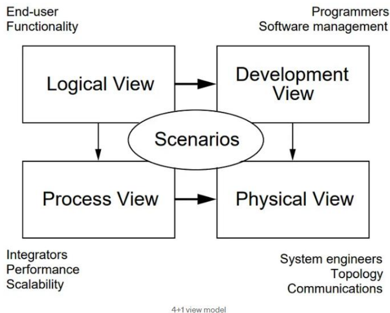
Figure 16 The "4+1" View Model by Kruchten
