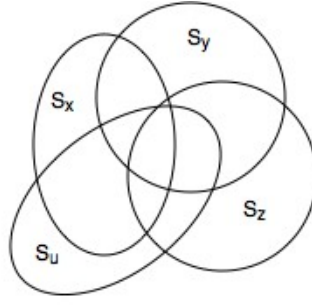
Figure 11.2: X = \bigcup_{x \in I} S_x . See Proposition 11.6.
