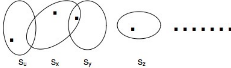
Figure 11.1: Axiom of Choice with choice function indicated by black dots.
