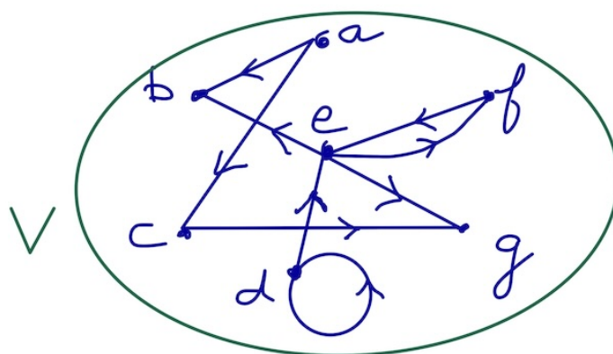
Figure 14.1: A very silly example of a \{V, \in\} structure. Read the arrow from a to b as “ b is a member of a ”. Probably no ZF axioms hold here.
