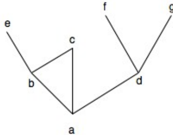
Figure 11.3: x \leq y if x = y or there is a “rising” path from x to y . For example, a \leq b , a \leq c and a \leq e .
